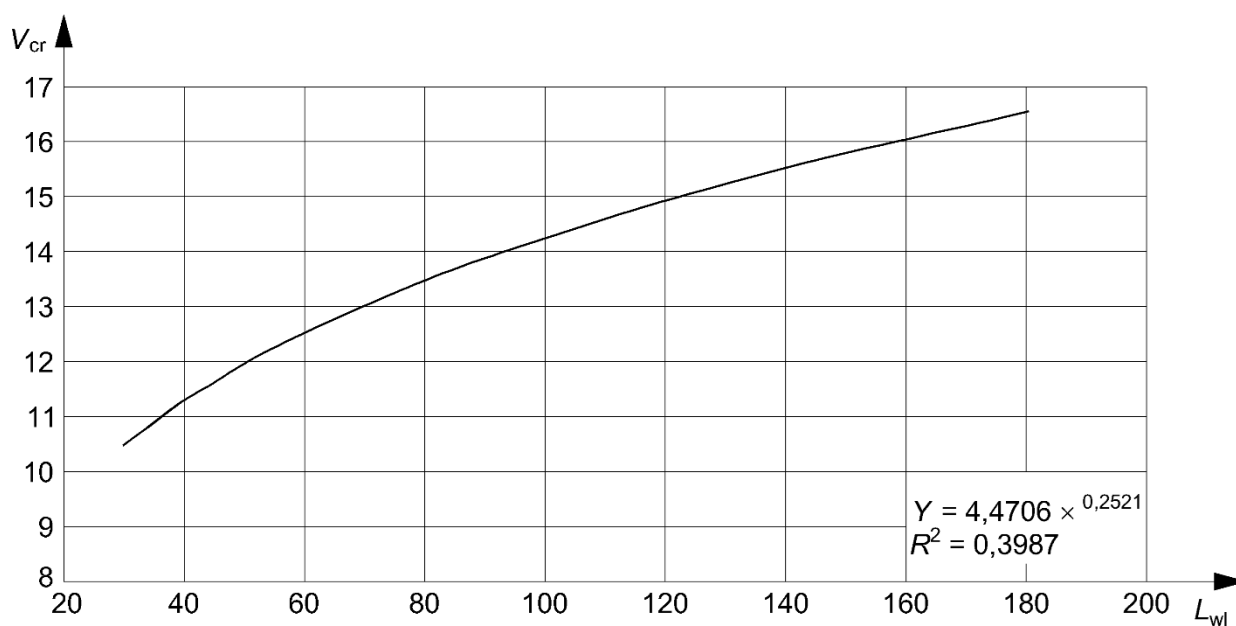
Figure A1: Speed vs. Length
